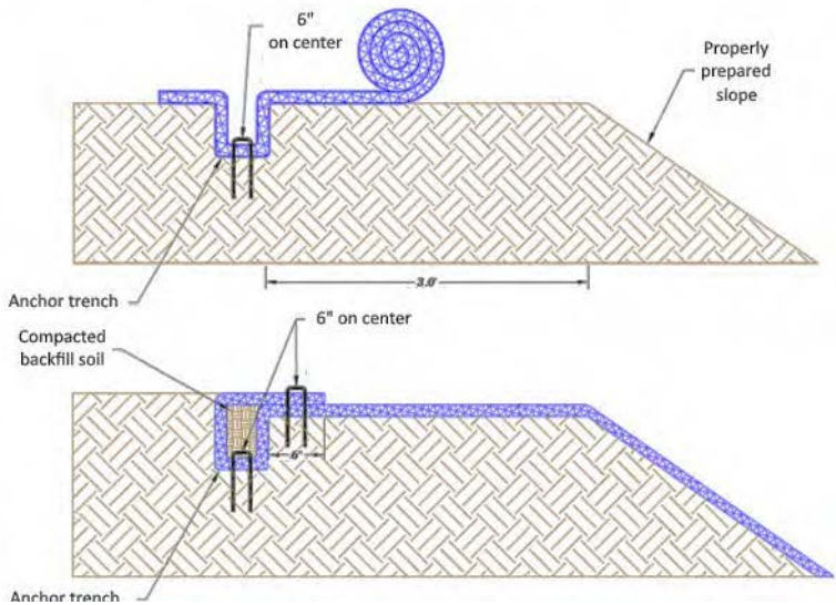
Method 2: Cover the keyed in area with a flap of the matting
