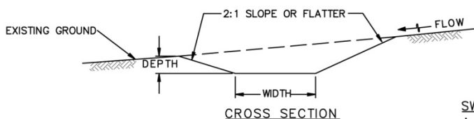
CROSS SECTION
