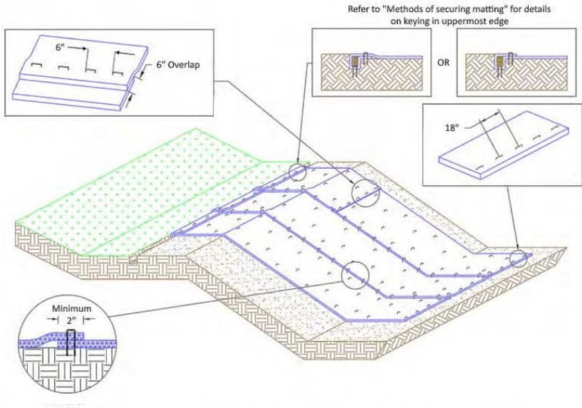
Installation of matting in a channel
