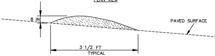
CROSS SECTION
