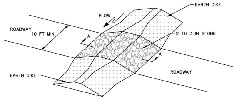
ISOMETRIC VIEW
