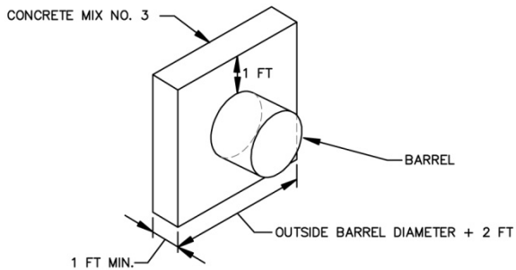
CONCRETE COLLAR DETAIL
