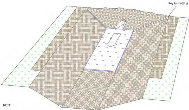
Installation of matting in a channel
