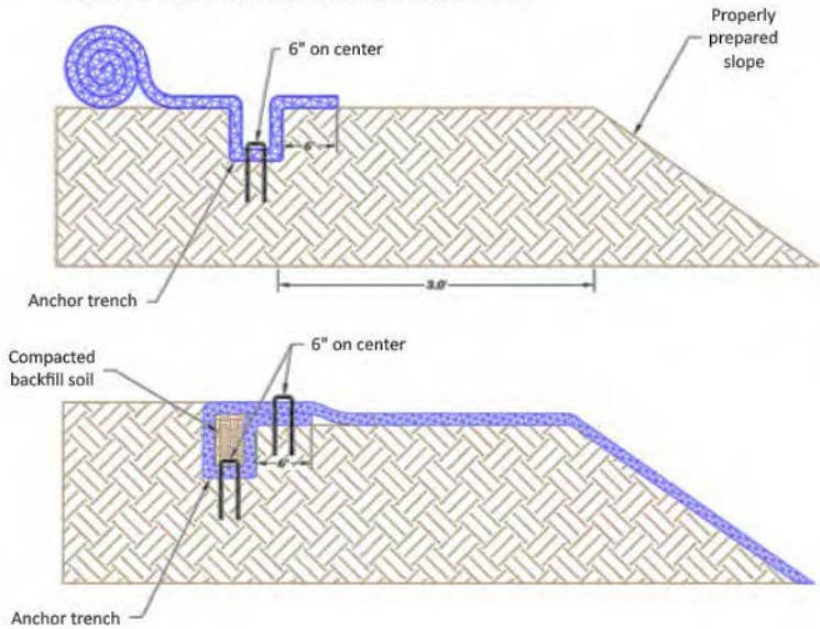
Method 1: Roll the matting over the keyed in area
