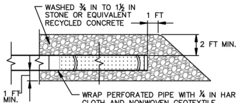
STONE ANCHOR DETAIL
