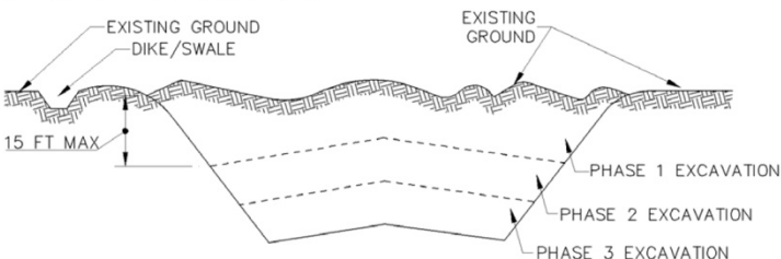
Figure B.1: Incremental Stabilization – Cut
