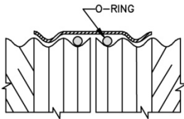
HUGGER (SEMI-CORRUGATED) BAND
