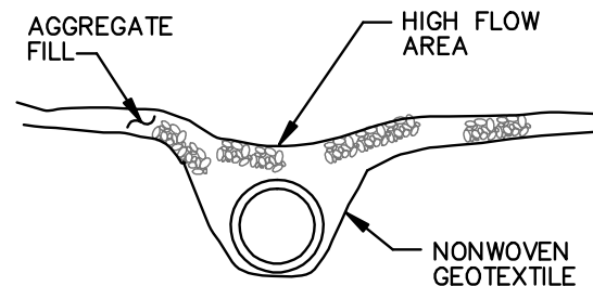
SINGLE PIPE
