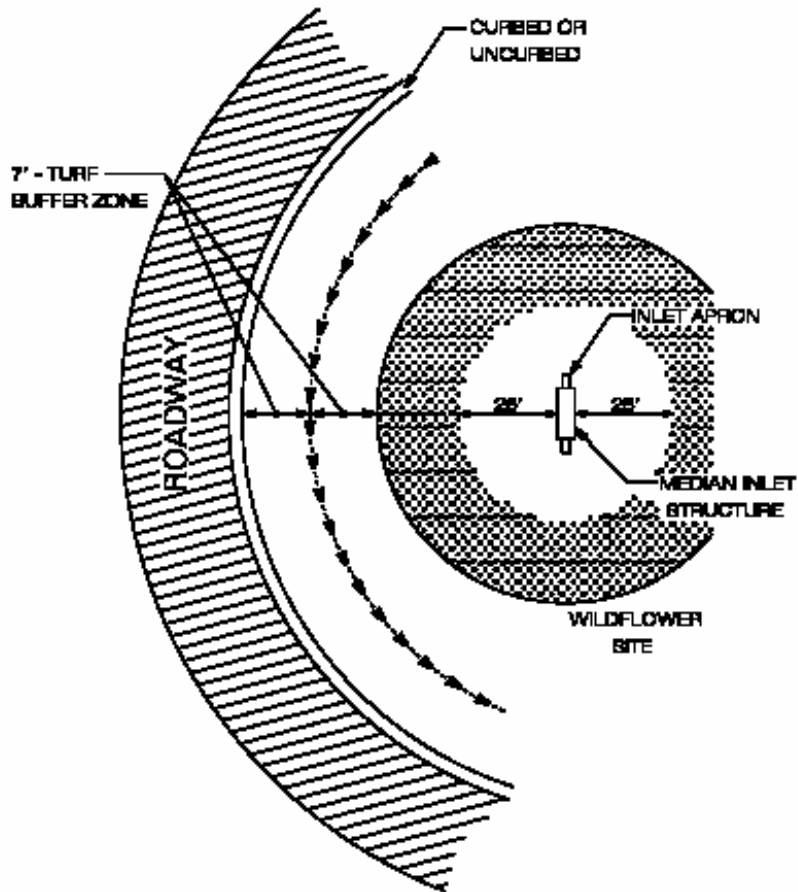
PLAN VIEW NO. 5 ROADSIDE RAMP - LESS THAN 4:1
