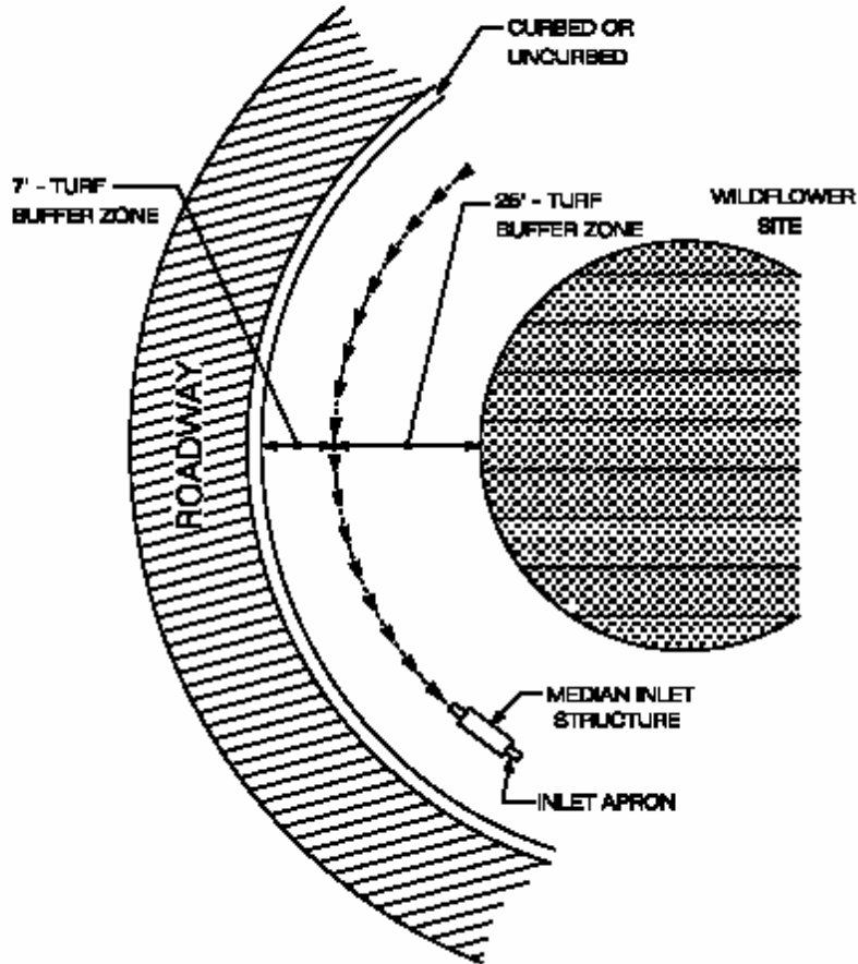
PLAN VIEW NO.6 ROADSIDE RAMP - STEEPER THAN 4:1
