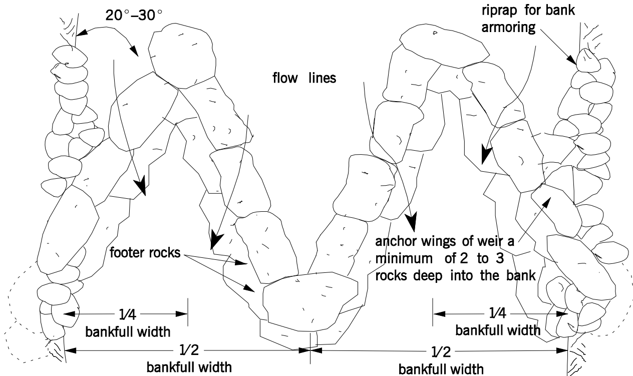
PLAN VIEW: W-ROCK WEIR
