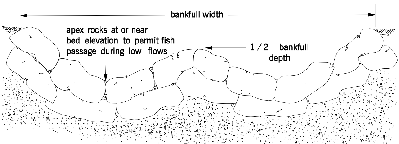
SECTION VIEW: W-ROCK WEIR
