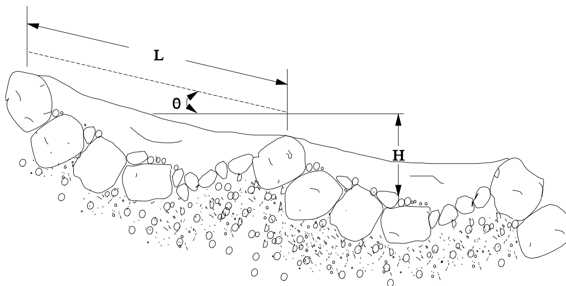
DEFINITION SKETCH: STEP POOL
