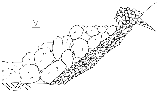
MGWC 2.1/2.5: fascine w/rock toe
