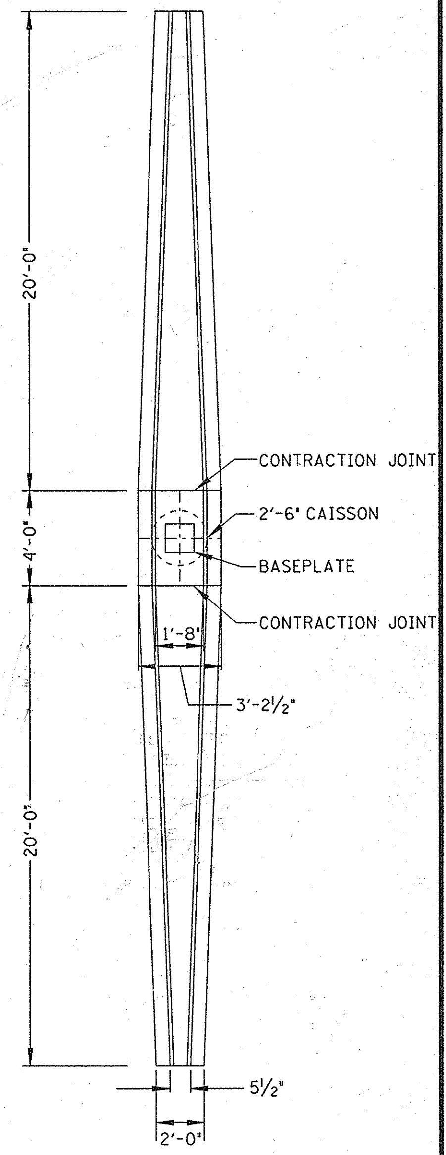
PLAN MEDIAN WIDENING DETAIL - TYPE J NOT TO SCALE
