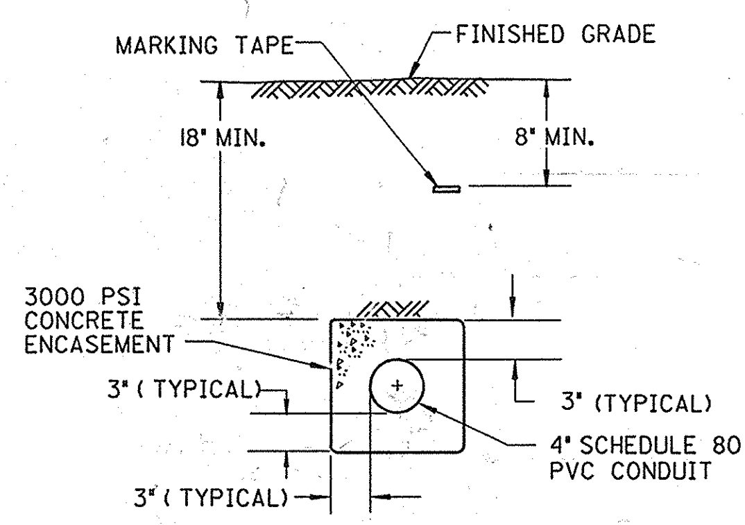
ONE WAY 4" CONCRETE ENCASED PVC CONDUIT NOT TO SCALE
