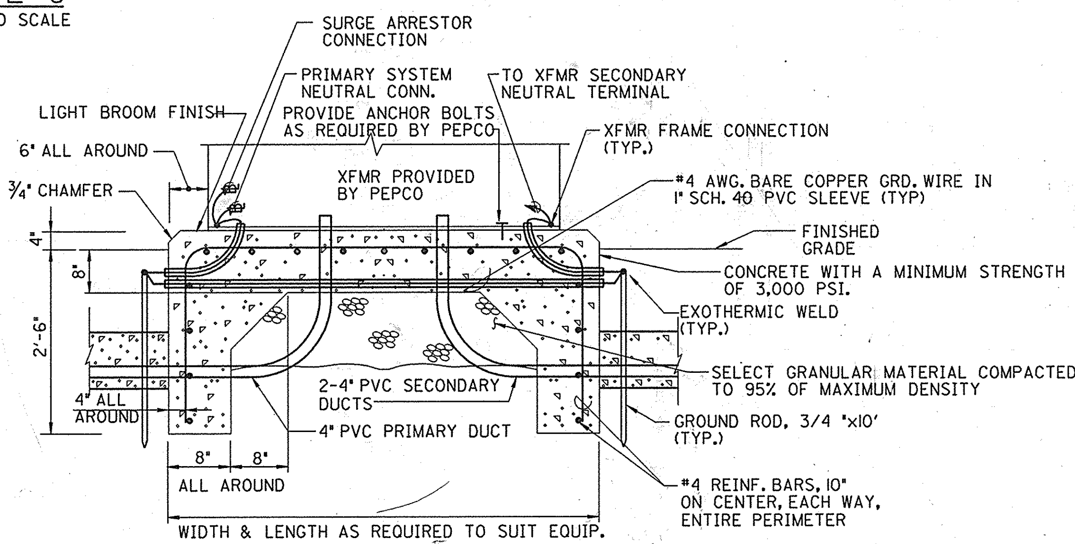
TRANSFORMER PAD DETAIL NOT TO SCALE
