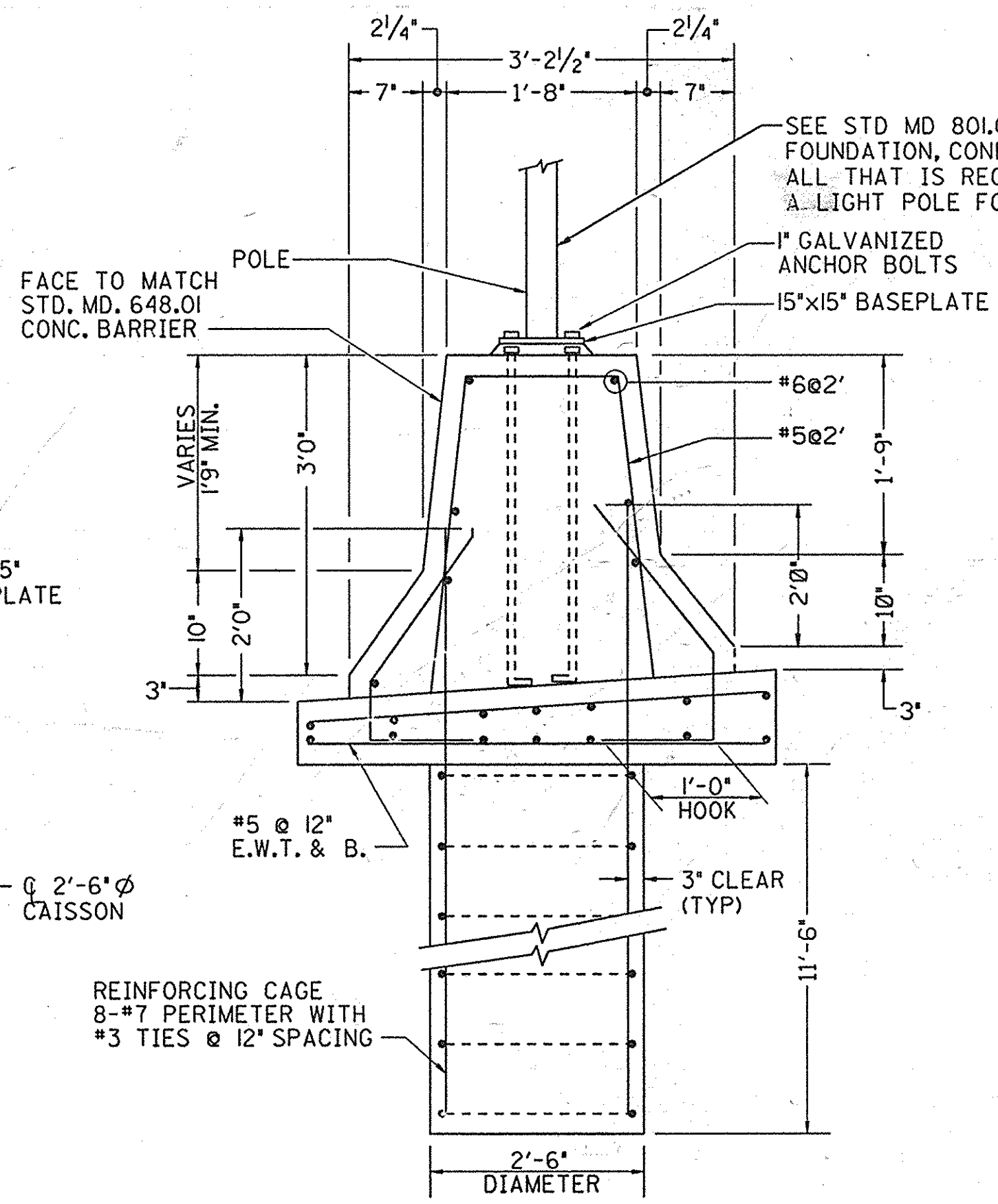
TYPICAL LIGHTING STRUCTURE FOUNDATION - TYPE J NOT TO SCALE
