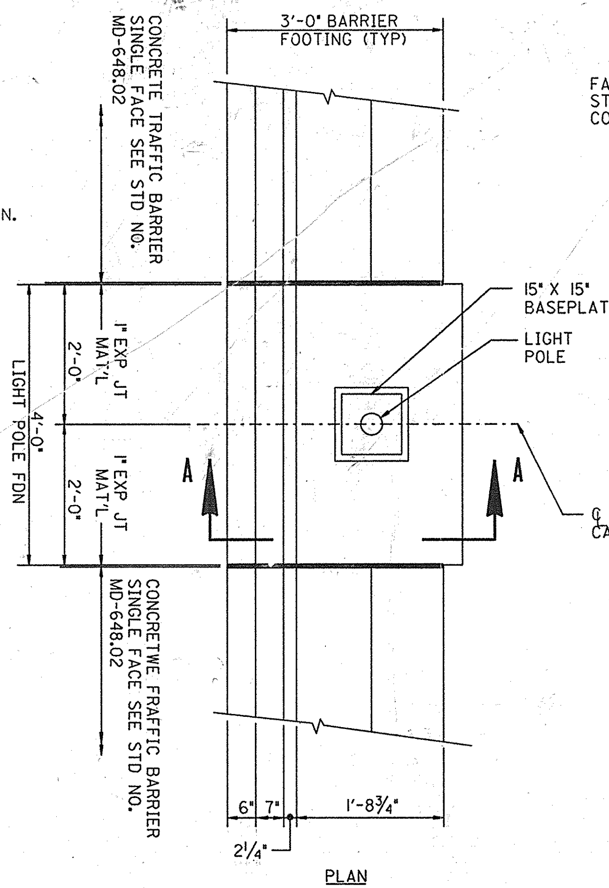
TYPICAL LIGHTING STRUCTURE FOUNDATION - TYPE J NOT TO SCALE
