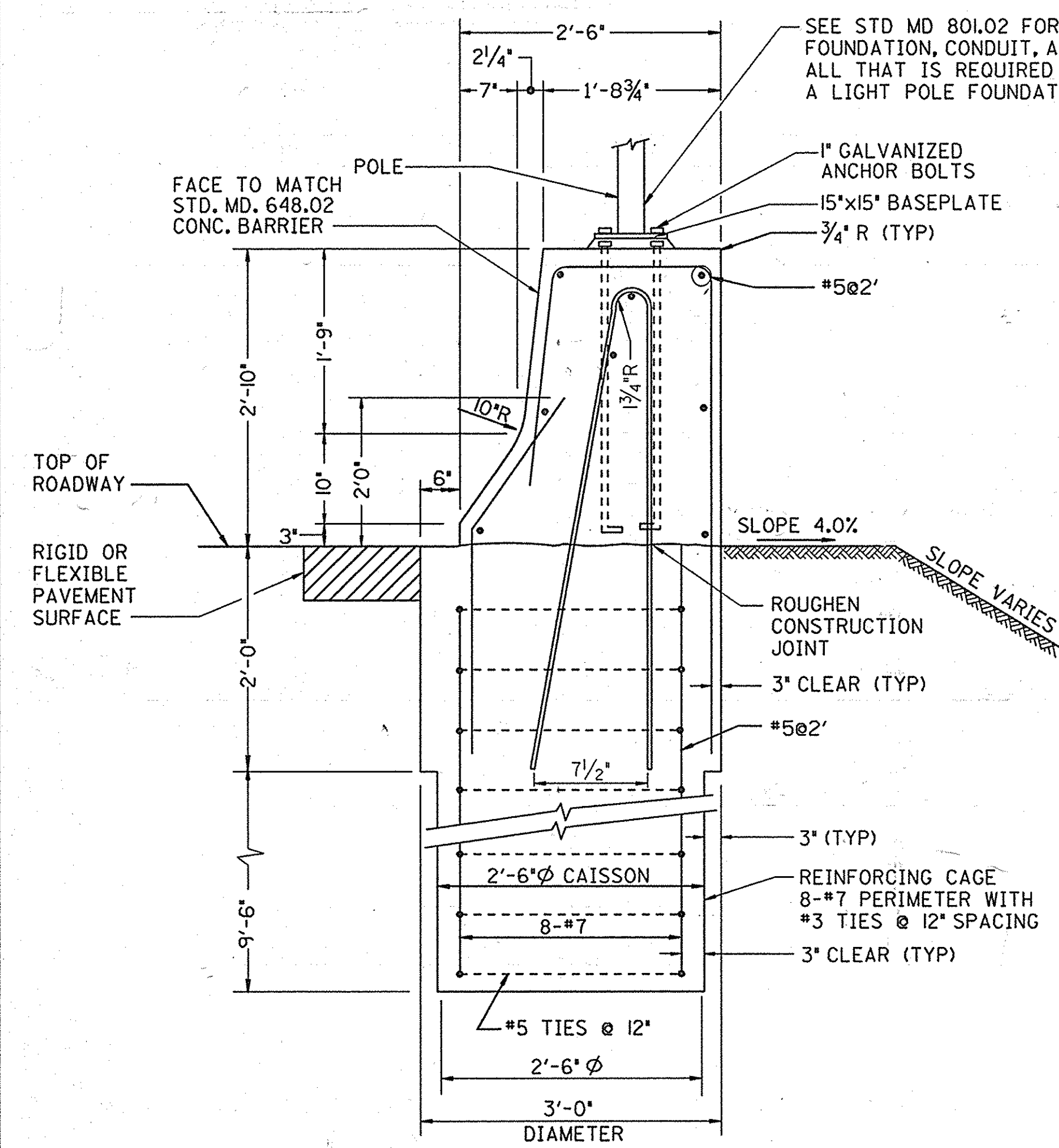
SECTION A-A LIGHT POLE FOUNDATION @ STANDARD SINGLE FACE TRAFFIC BARRIER TYPE C NOT TO SCALE
