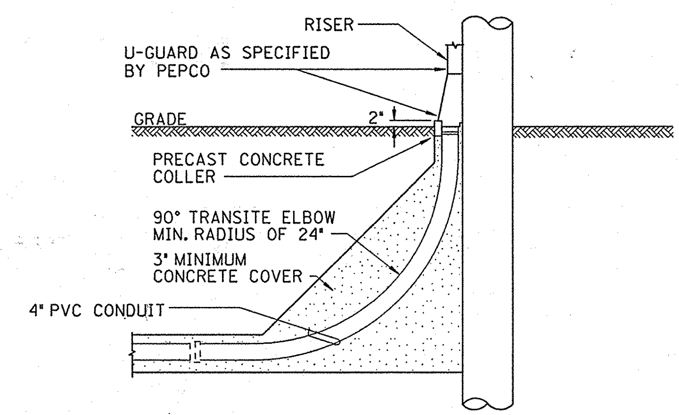
CONDUIT SWEEP DETAIL PEPCO UTILITY POLES NOT TO SCALE
