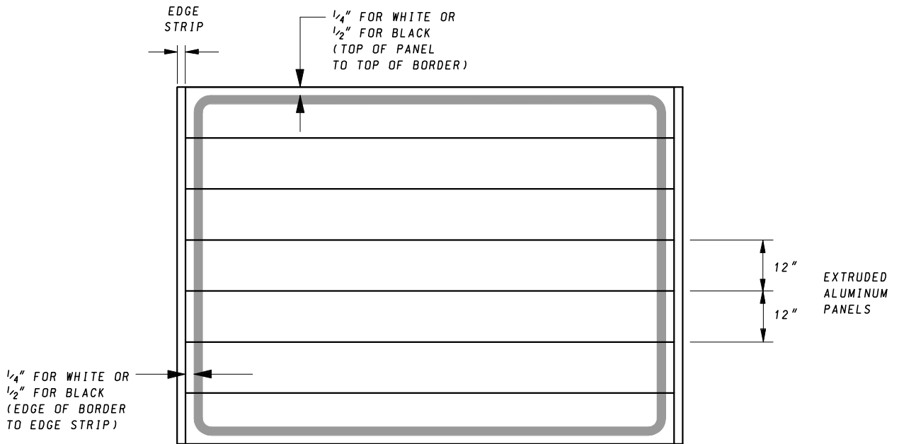
BORDER DETAIL
