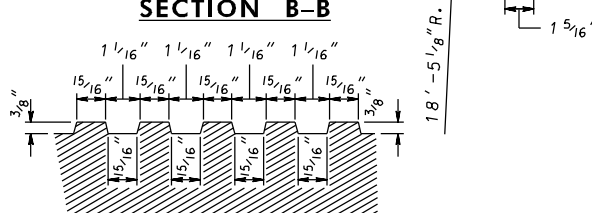
DETAIL OF CORRUGATIONS
