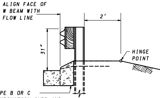
ALIGN FACE OF W BEAM WITH FLOW LINE TYPE B OR C COMBINATION CURB AND GUTTER OR TYPE B OR C CURB. * SEE NOTE 5
