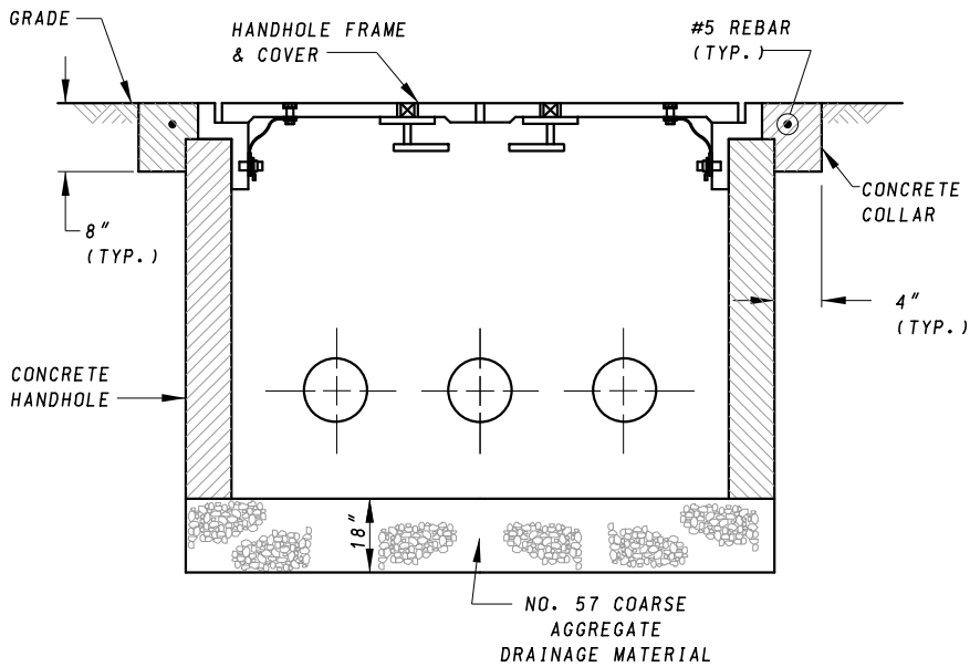
OVERSIZED HANDHOLE INSTALLATION DETAIL SECTION E - E
