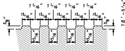
DETAIL OF CORRUGATIONS
