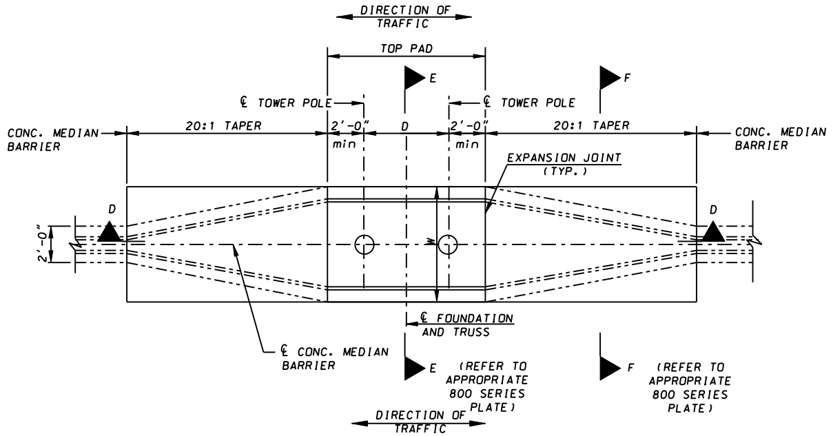
FOUNDATION PLAN TYPE "B"
