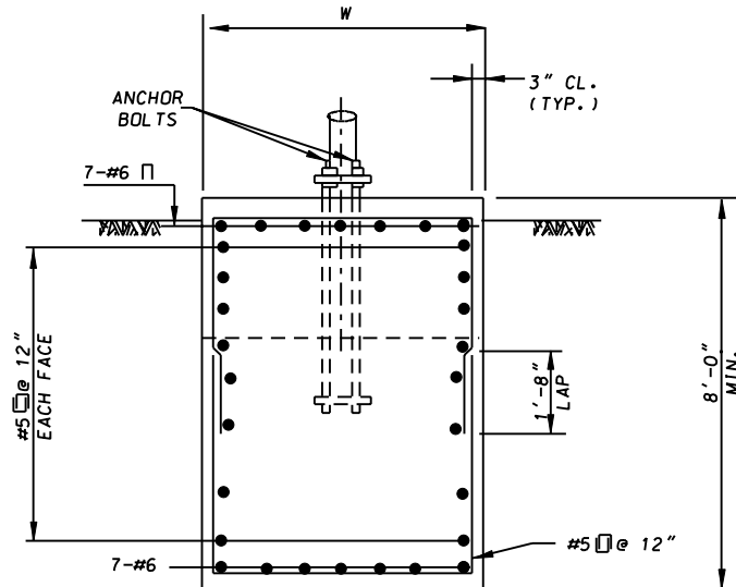
SECTION B-B (FROM 800 SERIES STANDARD)
