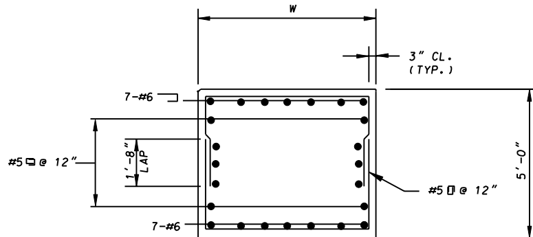
SECTION C-C (FROM 800 SERIES STANDARD)
