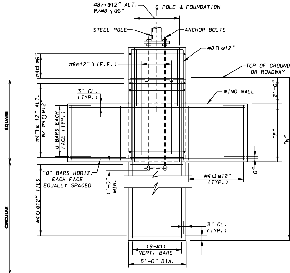
SECTION B-B
