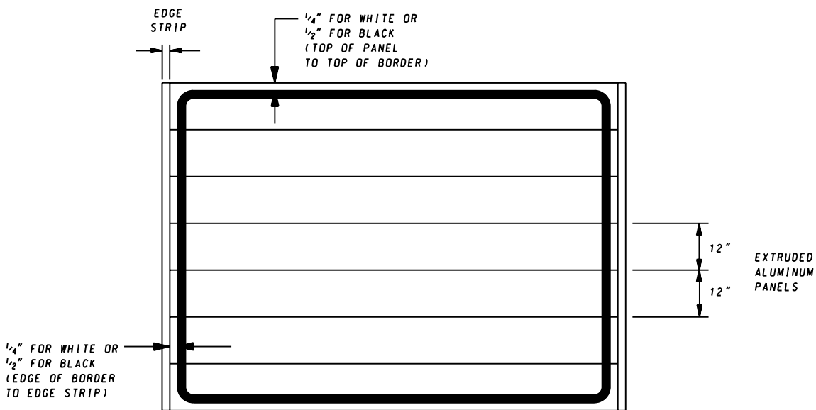
BORDER DETAIL
