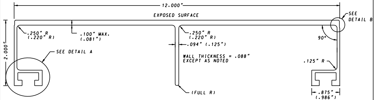
ALUMINUM PANEL - NOTCHED CORNERS (SEE NOTE 1)
