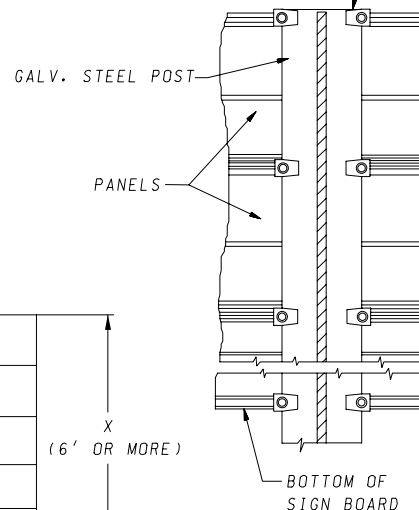
DETAIL A
