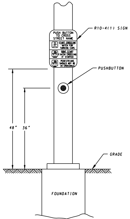
METAL POLE
