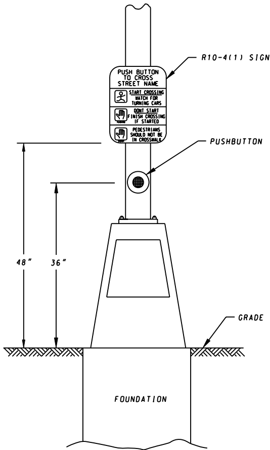
PEDESTAL POLE
