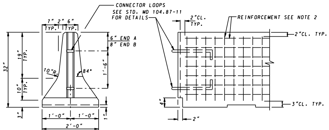
END VIEW
