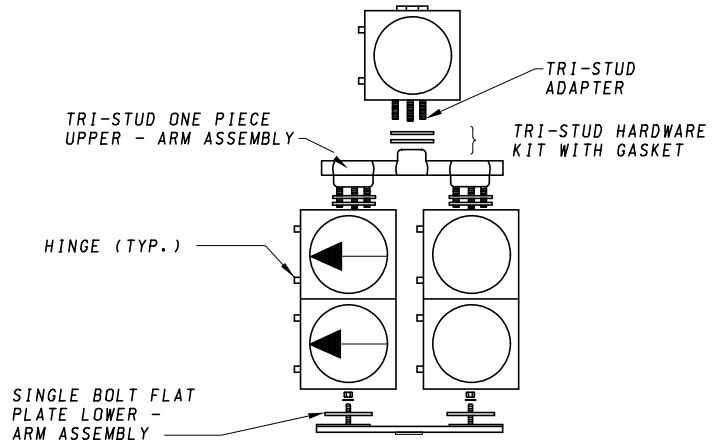
ONE-WAY, FIVE-SECTION 12" SIGNAL HEADS
