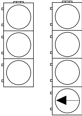
ONE-WAY THREE OR FOUR - SECTION 12" SIGNAL HEADS THREE - SECTION 12"/8" COMBINATIONS
