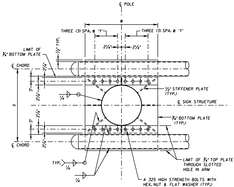
PLAN - POLE AND TRUSS ASSEMBLY
