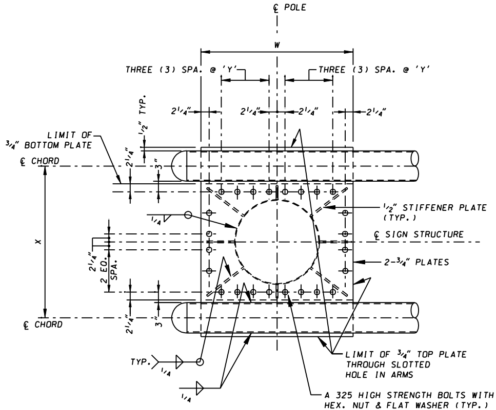
PLAN - POLE AND TRUSS ASSEMBLY
