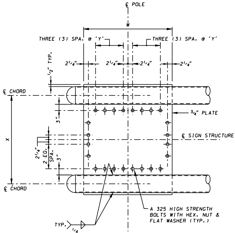
PLAN - TRUSS ASSEMBLY
