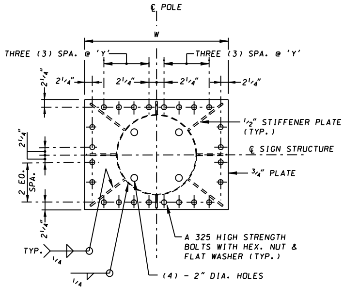
PLAN - POLE ASSEMBLY
