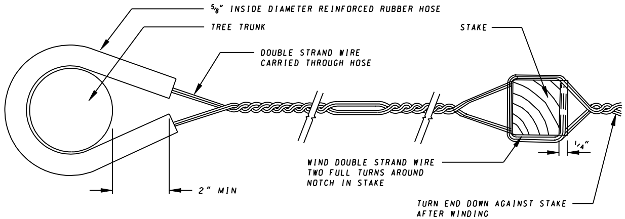
DOUBLE STRAND 14 GAUGE, GALVANIZED, WIRE FASTENER - TYPE B
