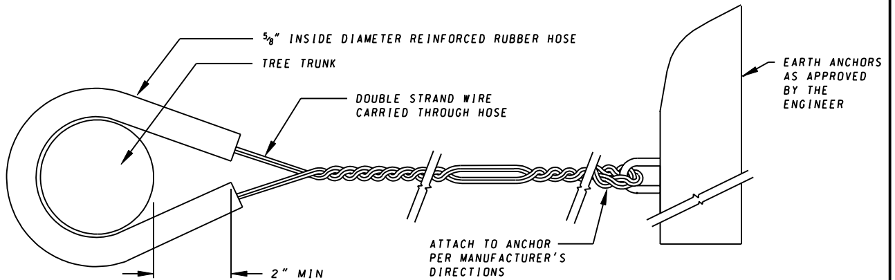
DOUBLE STRAND 12 GAUGE, GALVANIZED, WIRE FASTENER - TYPE C
