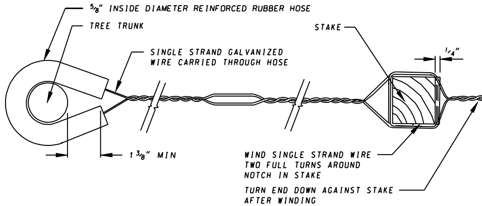
SINGLE STRAND 14 GAUGE, GALVANIZED, WIRE FASTENER - TYPE A
