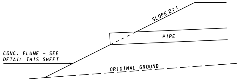
PIPE LOCATIONS UNDER DEEP FILL
