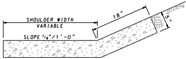
CONCRETE SHOULDER & REBUT
